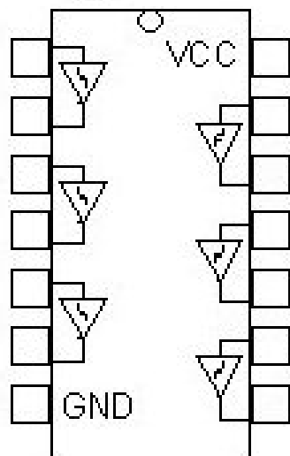
40106 Hex inverter trigger schmitt
